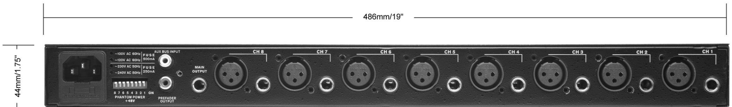
Back Panel
