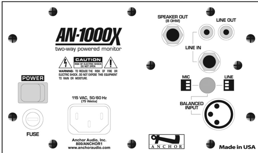
(AN-1000X Back Panel Shown)
